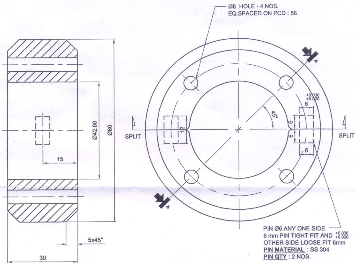
SECTION - AA
